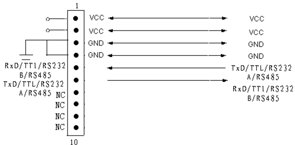
TDX-2000 MODULE CONNECT SKETCH MAP
